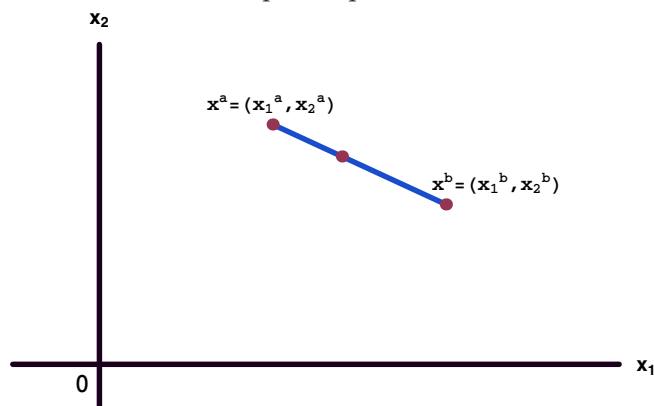
FIGURE 10. The Input Requirement Set is Convex
