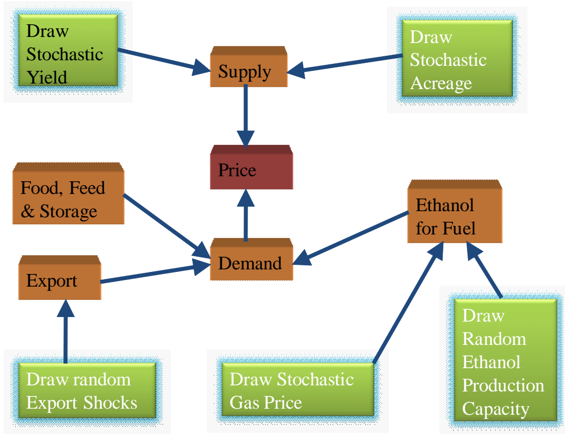
Figure 1: Stochastic corn supply and demand diagram
