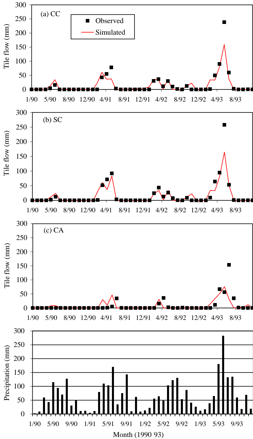
Figure 3. Observed and simulated monthly tile flows over 1990-93 at Lambertson, MN, after curve number calibration (CN2=65), for (a) CC, (b) SC, and (c) CA
