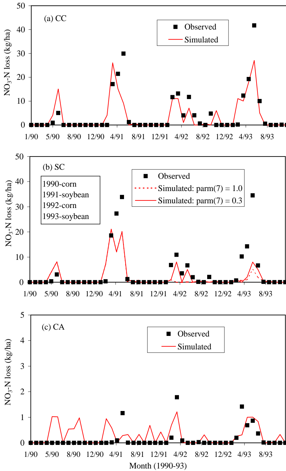
Figure 2. Observed and simulated monthly NO 3 -N losses over 1990-93 at Lamberton, MN, prior to curve number calibration (CN2=78), for (a) CC, (b) SC, and (c) CA
