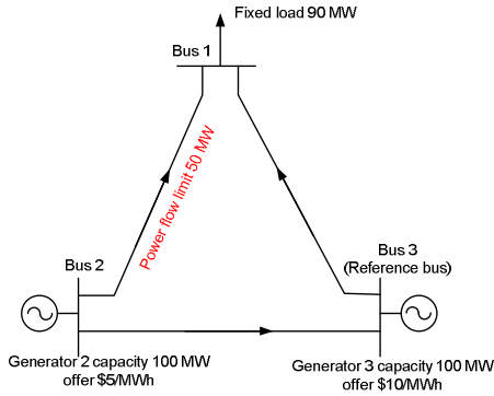
Fig. 1. LMP calculation for the full-structured DC OPF model
