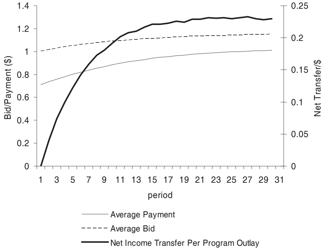
Figure 1: Some performance indicators for the discriminatory auction
