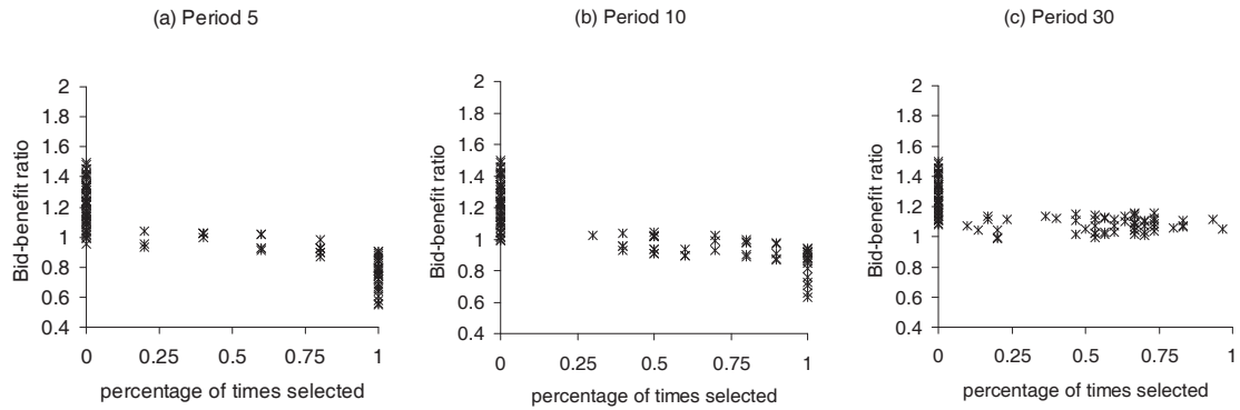
Figure 3. Bid-benefit ratio versus percentage of times that a bidder was selected.
